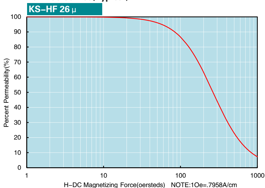
DC-Bias Curves(Typical)
